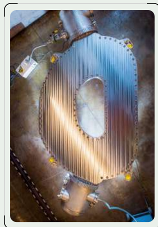
A FUSION MAGNET MANUFACTURED BY COMMONWEALTH FUSION SYSTEMS USING A NEW HIGH-TEMPERATURE SUPERCONDUCTOR
