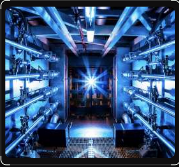
INSIDE OF A NIF PREAMPLIFIER SUPPORT STRUCTURE
